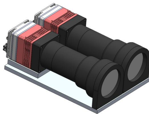
Figure 15: ACMEs FINIS instrument
