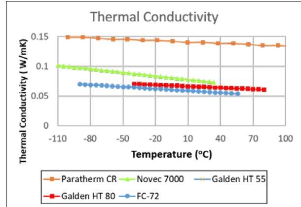
Figure 8: ACCS Working Fluid Comparison: Thermal Conductivity
