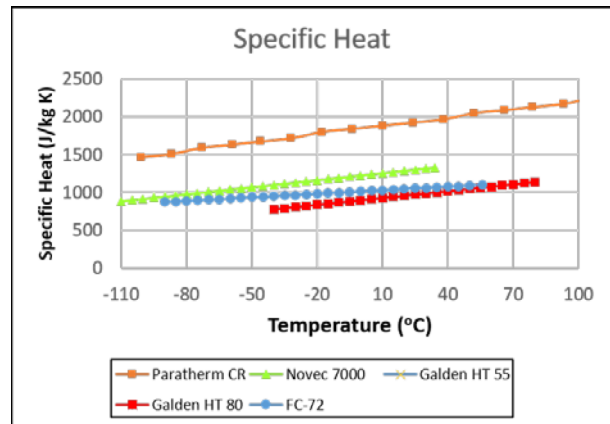
Figure 9: ACCS Working Fluid Comparison: Specific Heat
