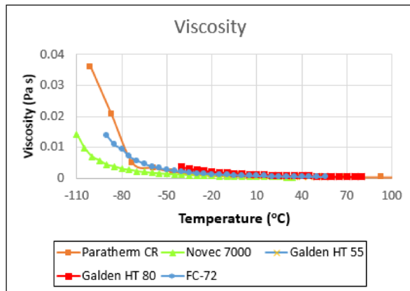
Figure 6: ACCS Working Fluid Comparison: Viscosity
