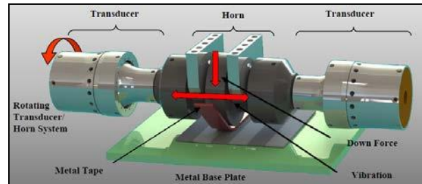
Figure 13: UAM Welding of Foil Tapes
