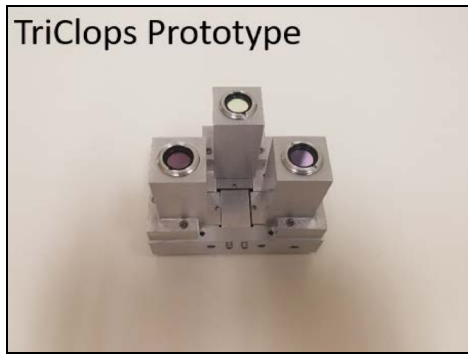
Figure 3: SABER-Lite “Tri-Clops” Radiometer Prototype
