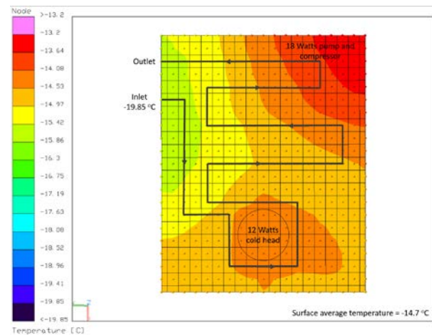
Figure 24: Thermal Desktop® Temperature Contour Plot of the ACCS HX for LM Micro Cryocooler
