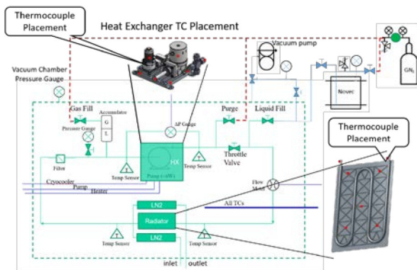
Figure 26: Schematic of the ACCS Characterization Test Setup
