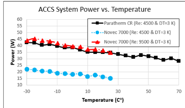
Figure 21: ACCS System Heat Rejection vs. Temperature for Paratherm CR & Novec 7000
