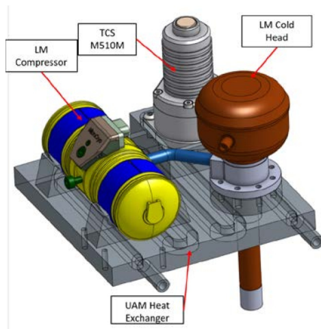
Figure 6: ACCS UAM HX Design for the LM Micro Cryocooler
