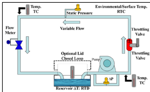
Figure 4: TCS M410 & M510 Pump Characterization Test Bed Schematic
