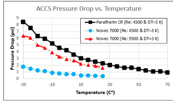
Figure 20: ACCS System Pressure Drop vs. Temperature for Paratherm CR & Novec 7000
