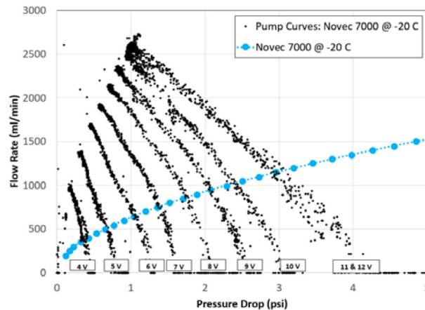
Figure 5: ACCS System Impedance Curve Overlaid on the Measured TCS M410 Pump Characterization Curves 15
