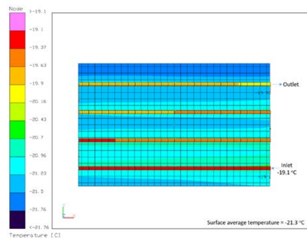
Figure 10: Thermal Desktop® Temperature Contour Plot of the ACCS Radiator Panel
