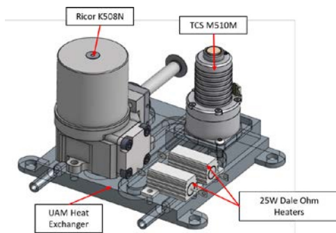
Figure 7: ACCS UAM HX Design for the Ricor K508N Cryocooler
