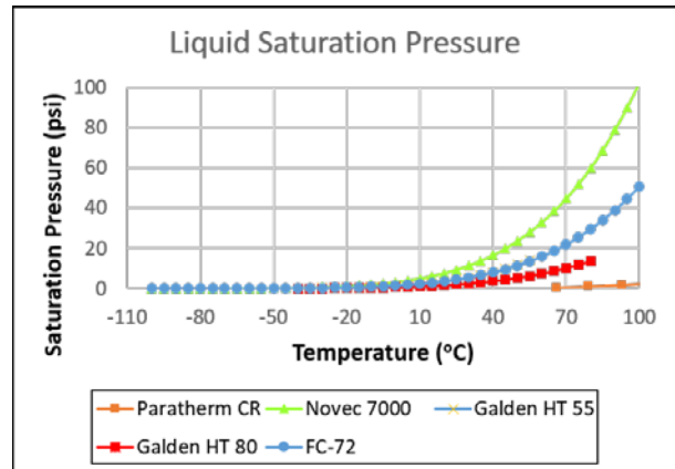
Figure 10: ACCS Working Fluid Comparison: Liquid Vapor Pressure
