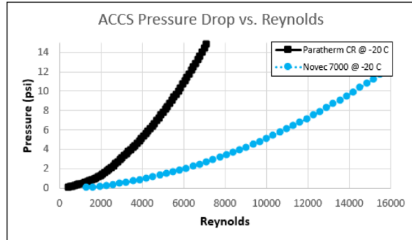
Figure 92: ACCS System Pressure Drop vs. Reynolds Number for Paratherm CR & Novec 7000
