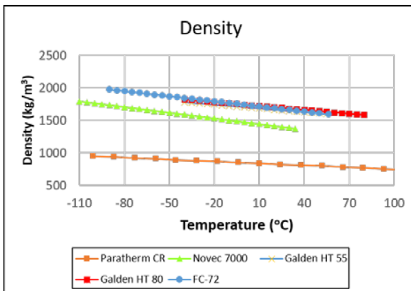
Figure 7: ACCS Working Fluid Comparison: Density
