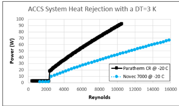
Figure 23: ACCS System Heat Rejection vs. Reynolds for Paratherm CR & Novec 7000
