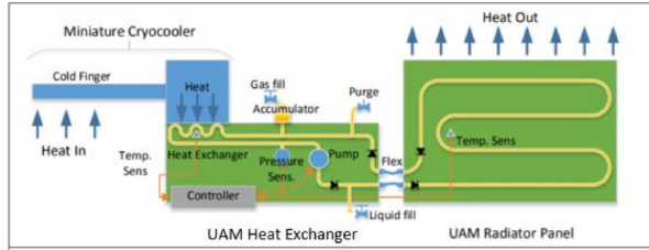
Figure 1: ACCS MPFL Thermal Accommodation of a Cryocooler
