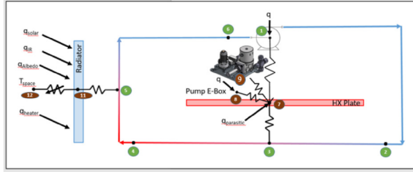
Figure 19. Simple Nodalized Model of the MPFL System.
