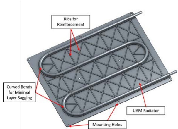
Figure 8: ACCS UAM Radiator Panel Design
