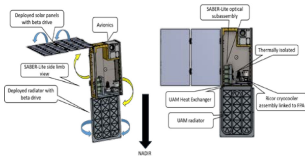
Figure 4: ACCS Accommodation of SABER-Lite Reference Mission
